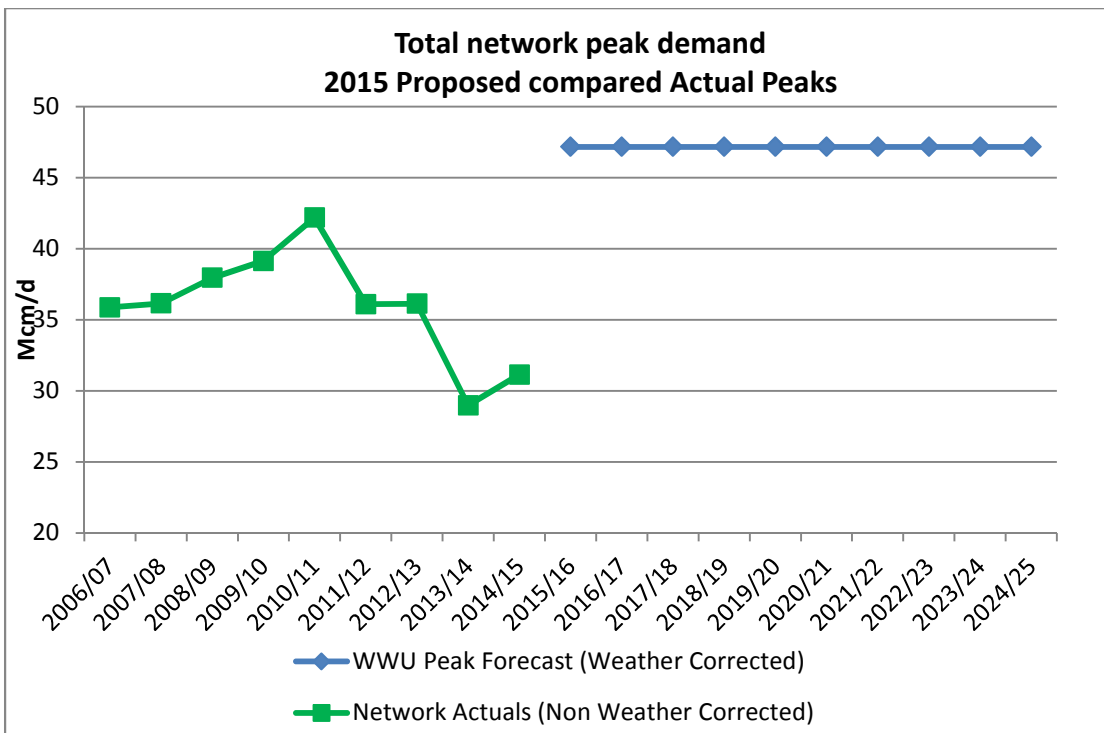
Figure 3.6: Forecast Peak Day Demand – 2013 Proposed compared to Actual Maximum Demand
