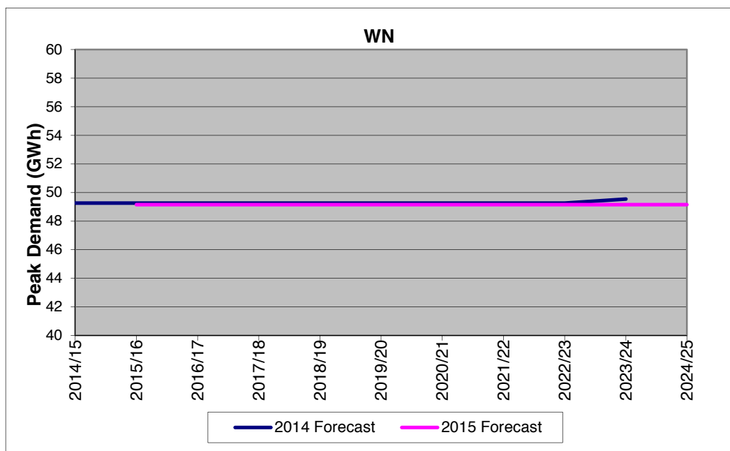
Figure 3.12: A Comparison of Peak Demand Forecasts for Wales North LDZ
